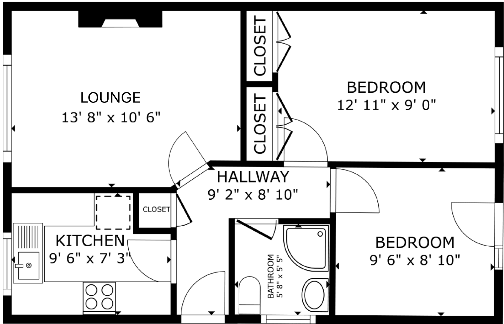
FLOOR PLAN
